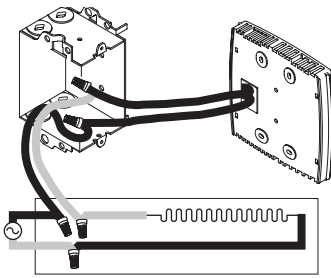
2-wire Installation
