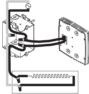
4-wire Installation
